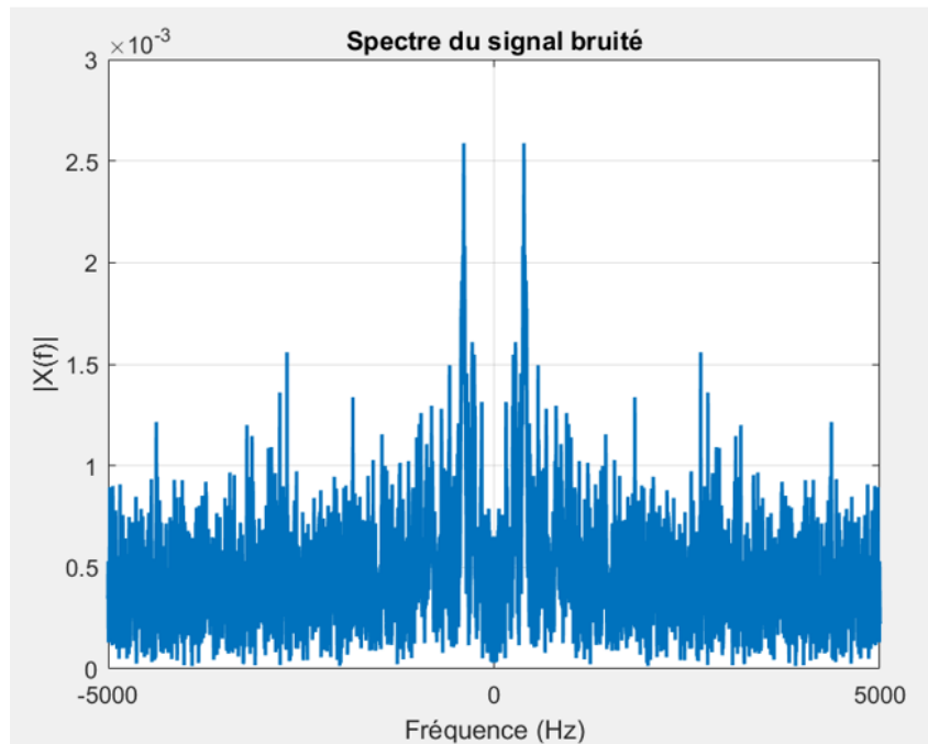
Figure 3: Frequency spectrum of the noisy signal showing both useful and noise components.
