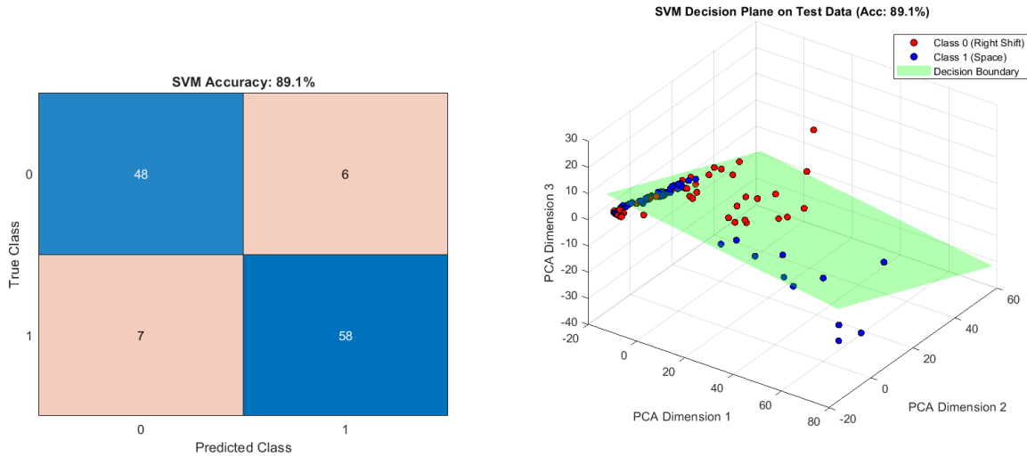
Figure 9: Confusion matrix and 3D visualization of binary separability
