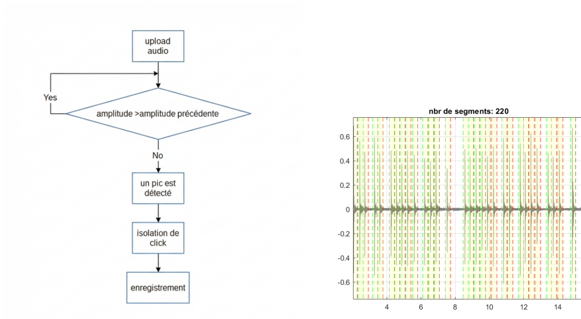
Figure 7: Principle flowchart and segmented peak isolation plot
