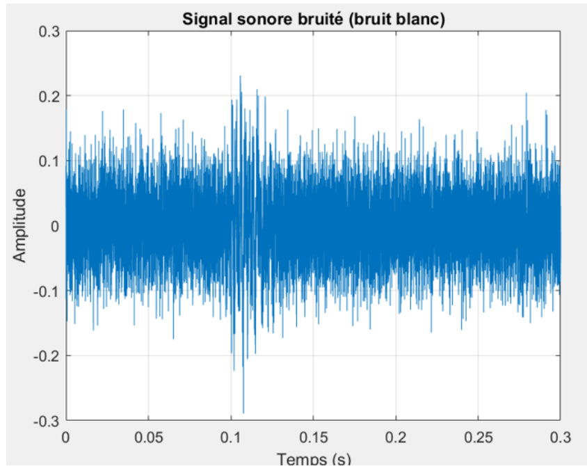
Figure 2: Raw captured signal containing keystroke transients buried in ambient noise.
