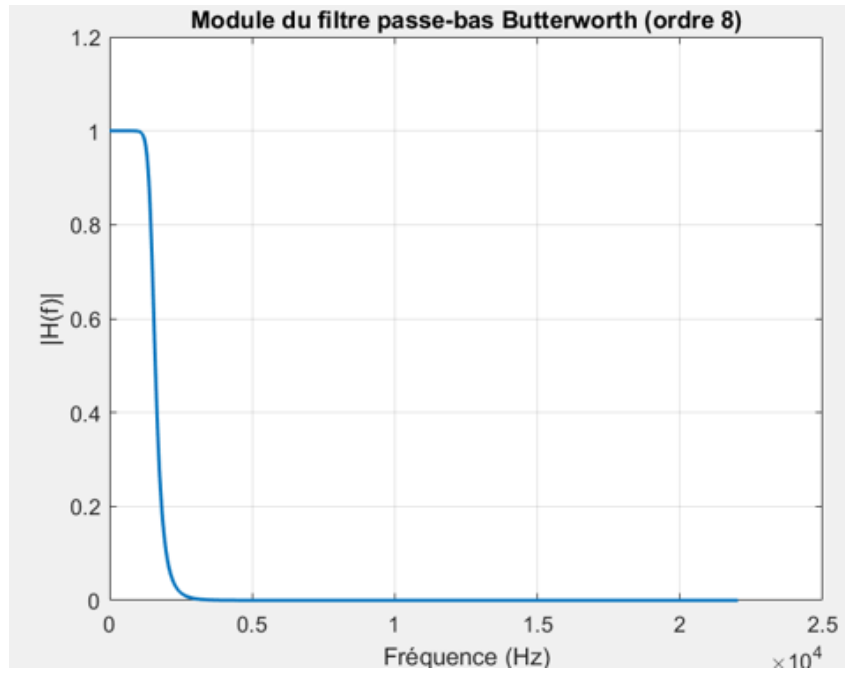
Figure 4: Frequency response of the Butterworth low-pass filter.
